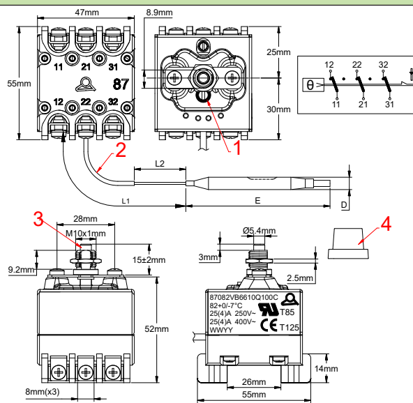
1. Sealing; 2. Sleeve; 3. Manual reset button; 4. Plastic cap(Black)
